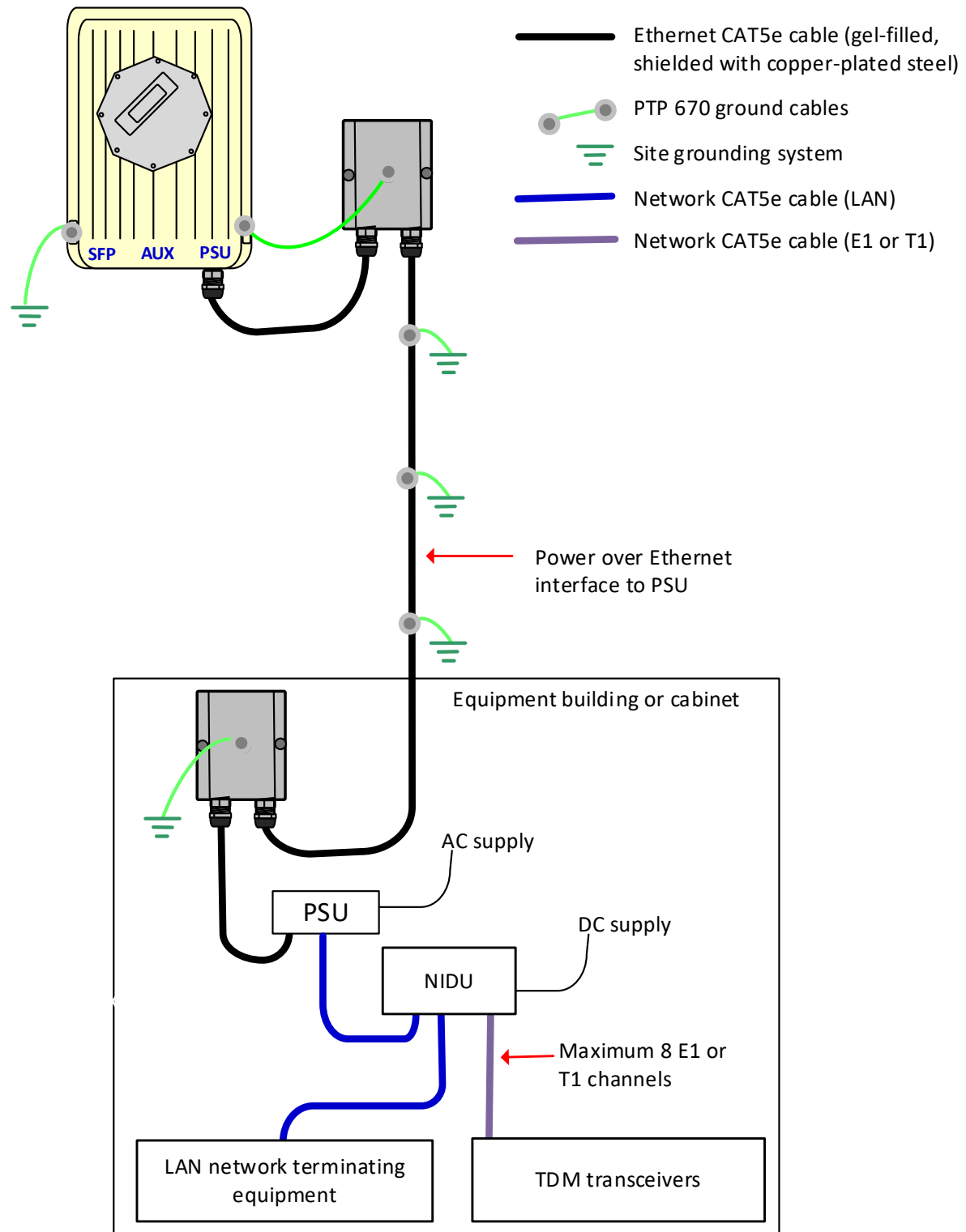
Figure 31 ODU with E1 or T1 interfaces
