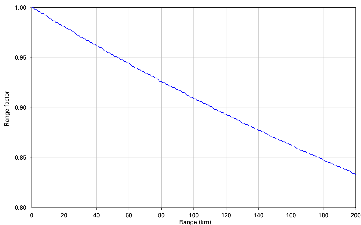
Figure 72 Range adjustment for PTP 670, symmetry 2:1, optimization IP, bandwidth 40 MHz
