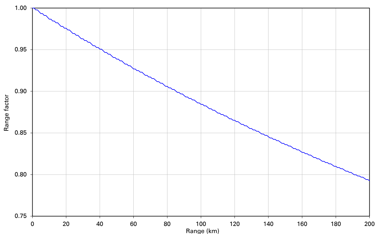
Figure 94 Range adjustment for PTP 670, adaptive, optimization IP, bandwidth 30 MHz
