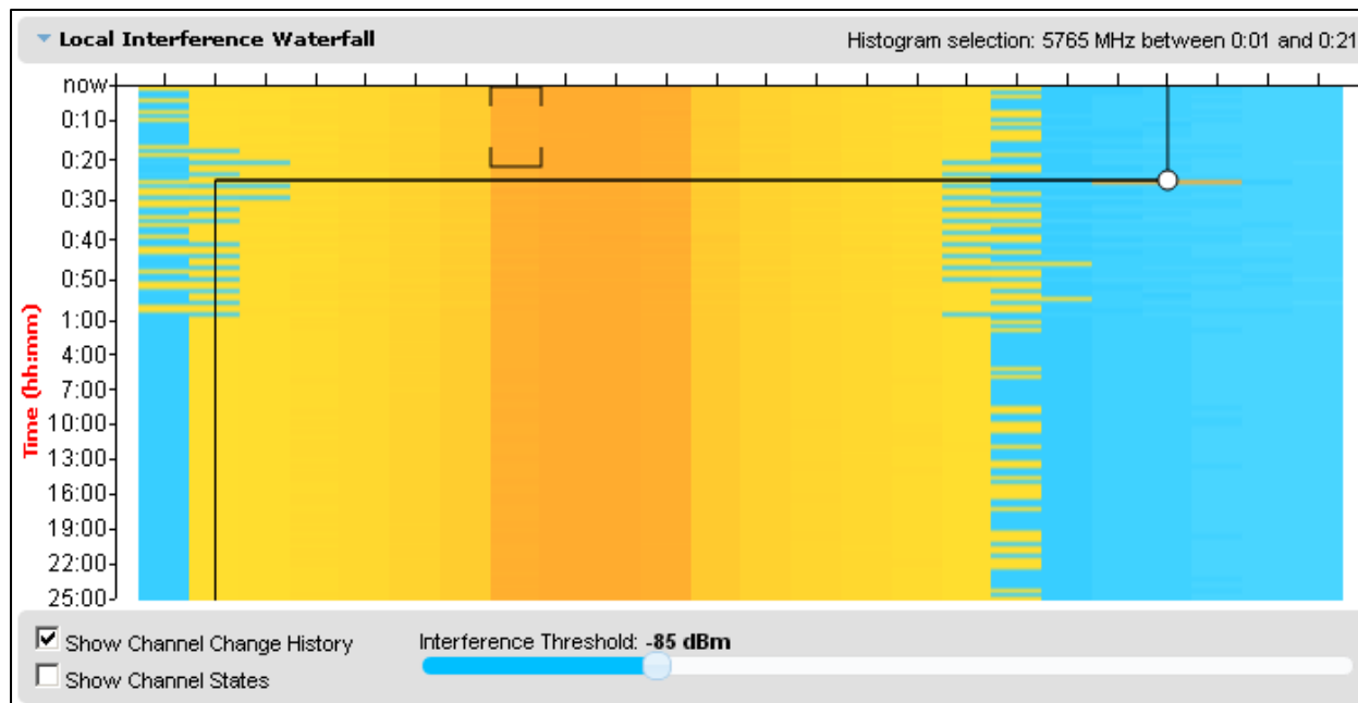
Figure 194 Spectrum Expert, Interference Waterfall plot
