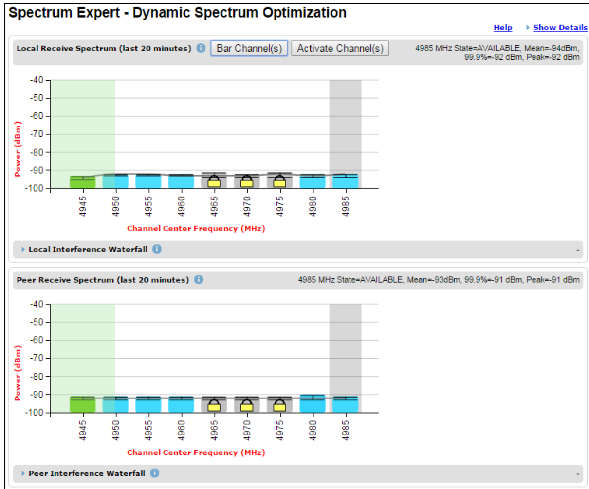
Figure 191 Barred channels
