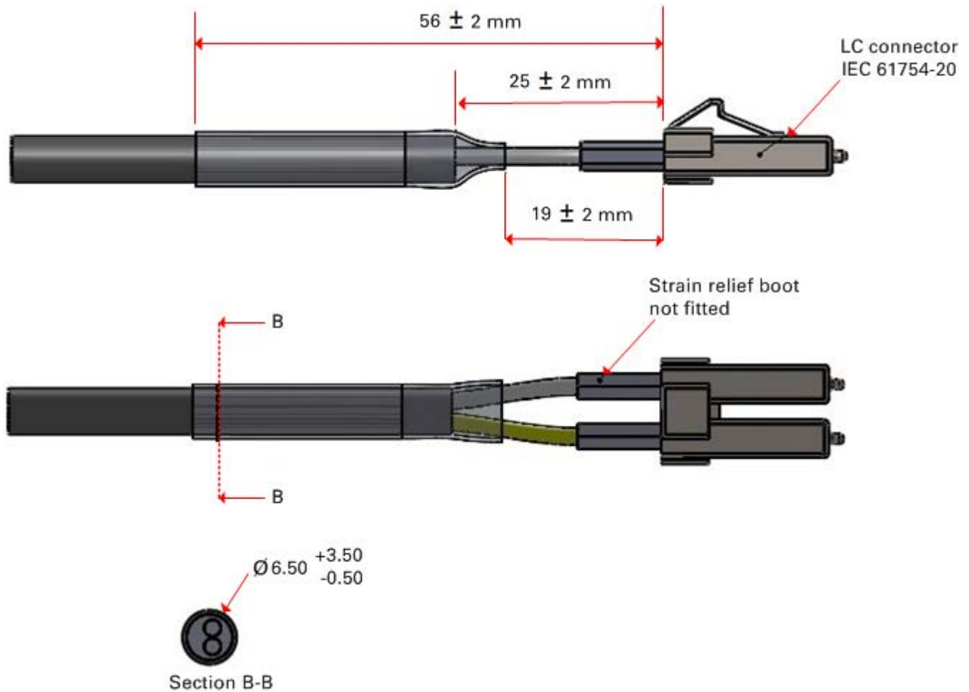
Figure 20 Optical optic cable and connector specification
