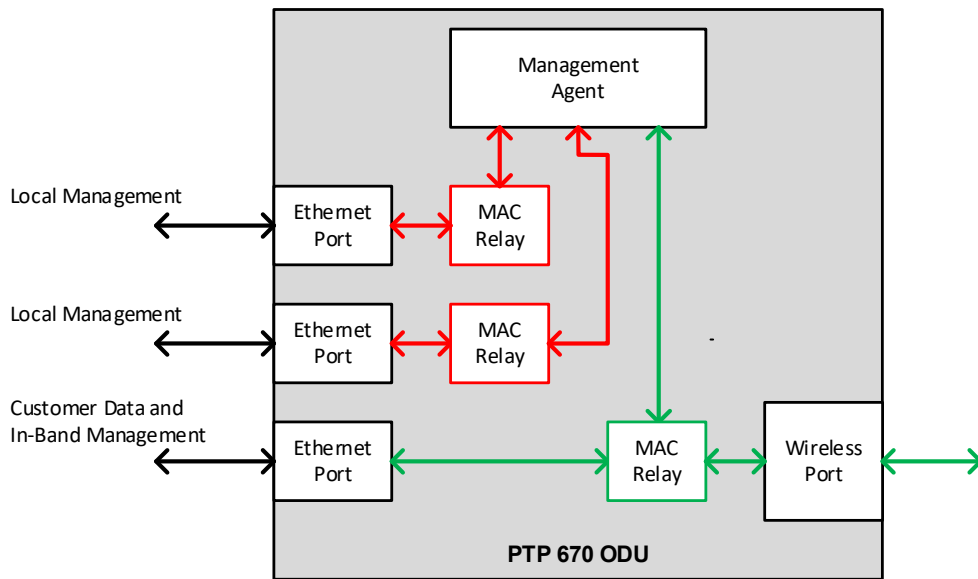
Figure 48 Ports and Services: Data + In-Band Management + Local Management + Local Management
