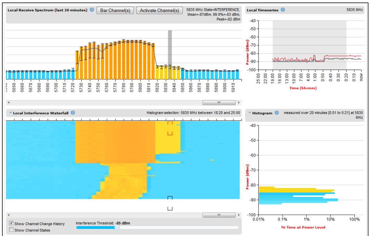
Figure 201 Spectrum Expert, example 4
