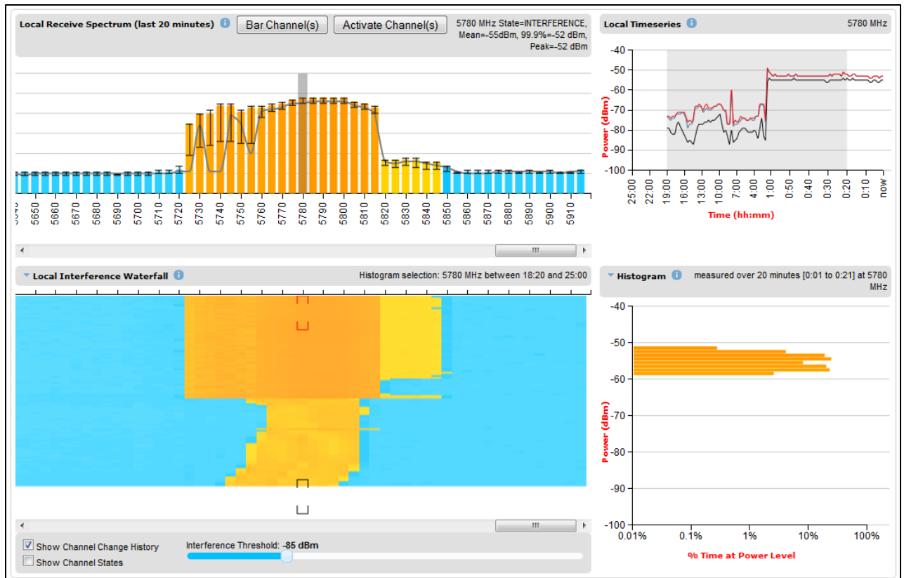
Figure 200 Spectrum Expert, example 3
