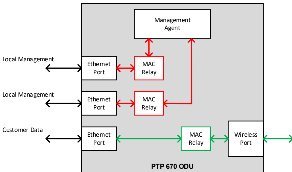
Figure 45 Ports and Services: Data + Local Management + Local Management
