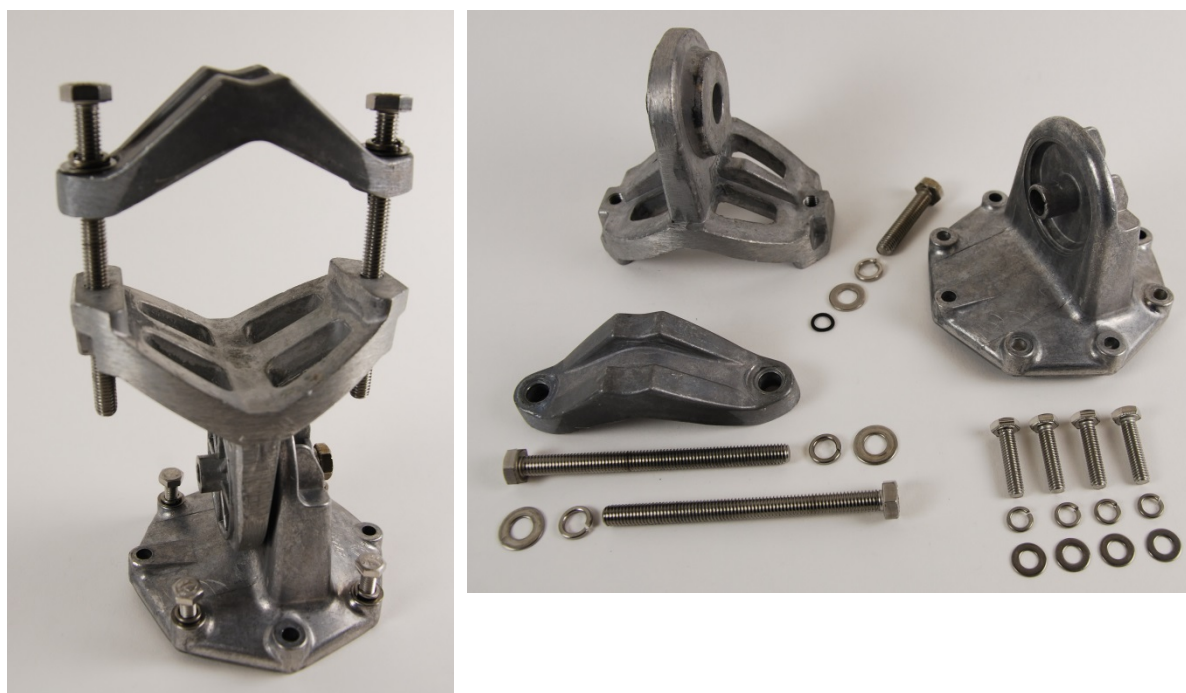
Figure 8 ODU Mounting Bracket (Integrated)
