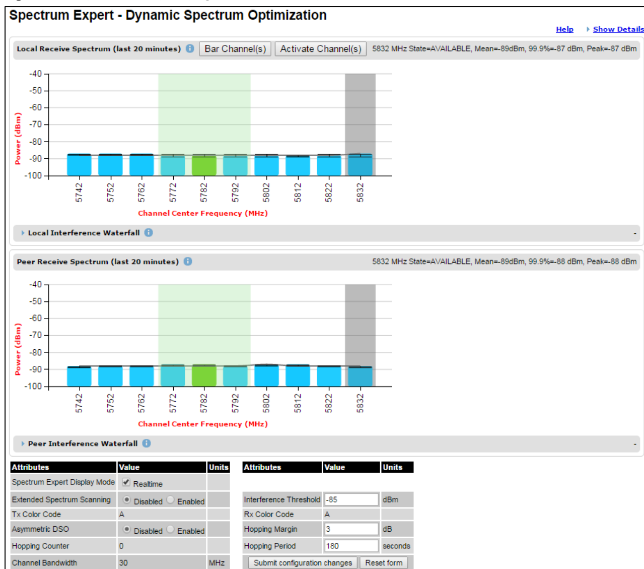
Figure 179 Spectrum Expert page – Standard Display mode
