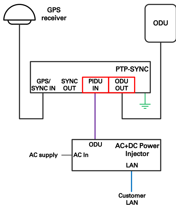
Figure 41 TDD synchronization configuration – single link with PTP-SYNC
