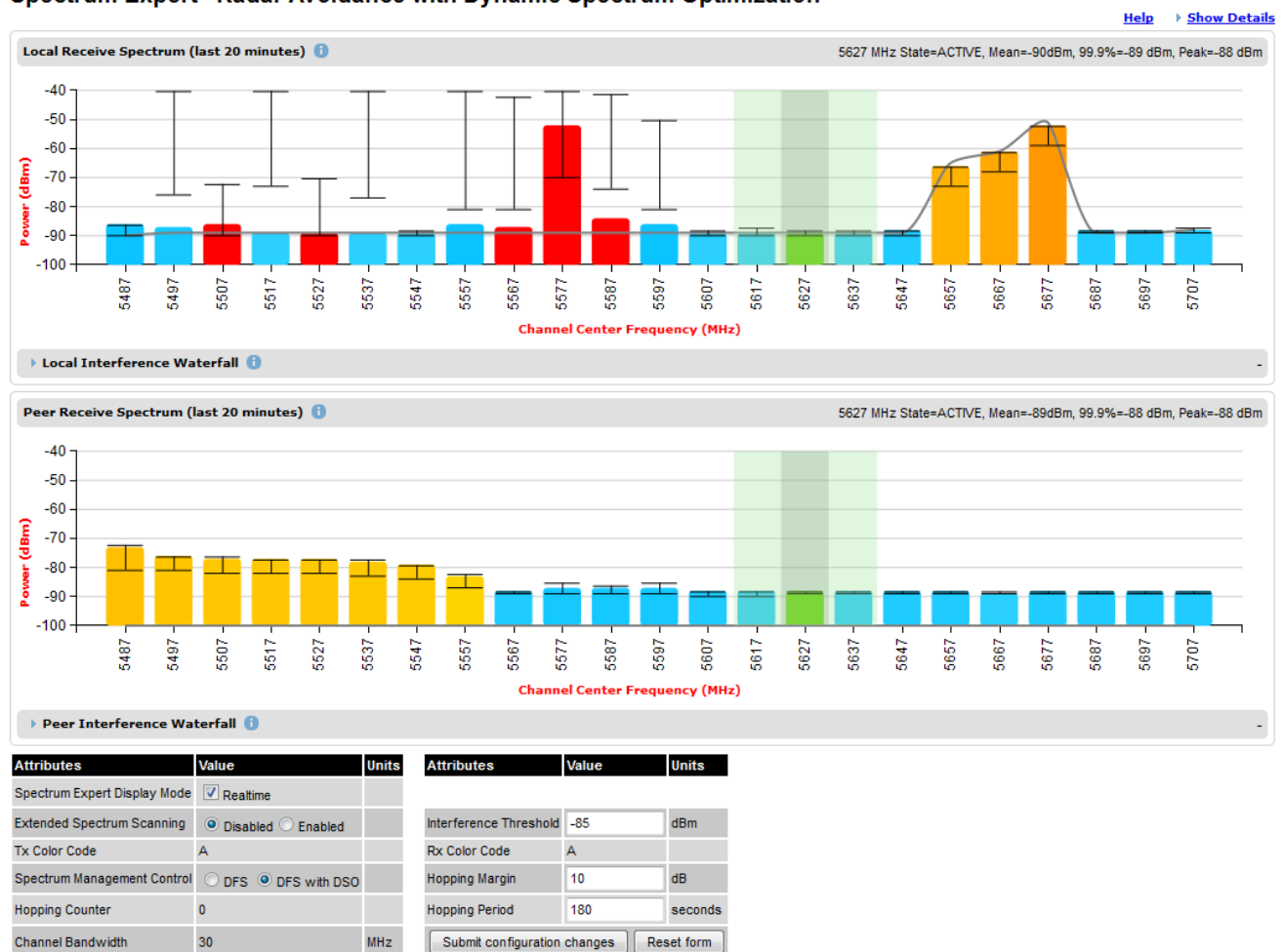
Figure 187 Spectrum Expert page with radar avoidance – Standard Display
