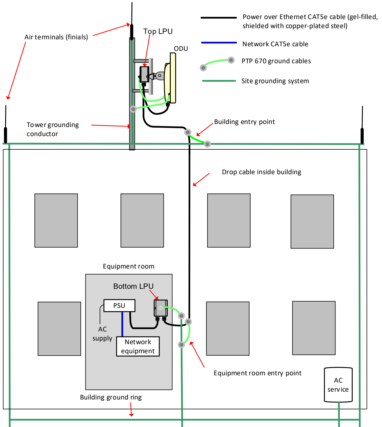
Figure 30 Roof installation
