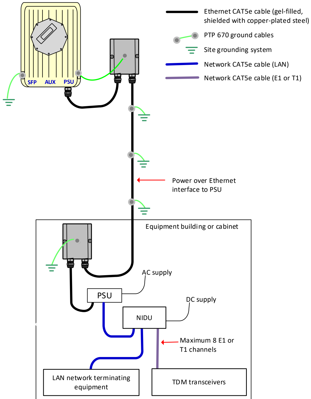
Figure 31 ODU with E1 or T1 interfaces
