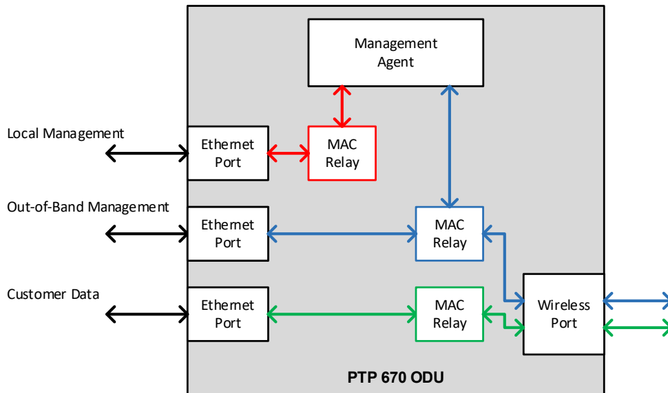
Figure 50 Ports and Services: Data + Out-Of-Band Management + Local Management
