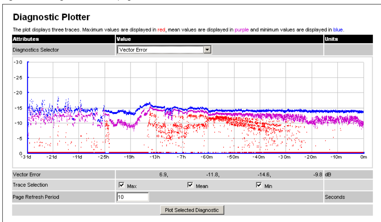
Figure 210 Diagnostic Plotter page
