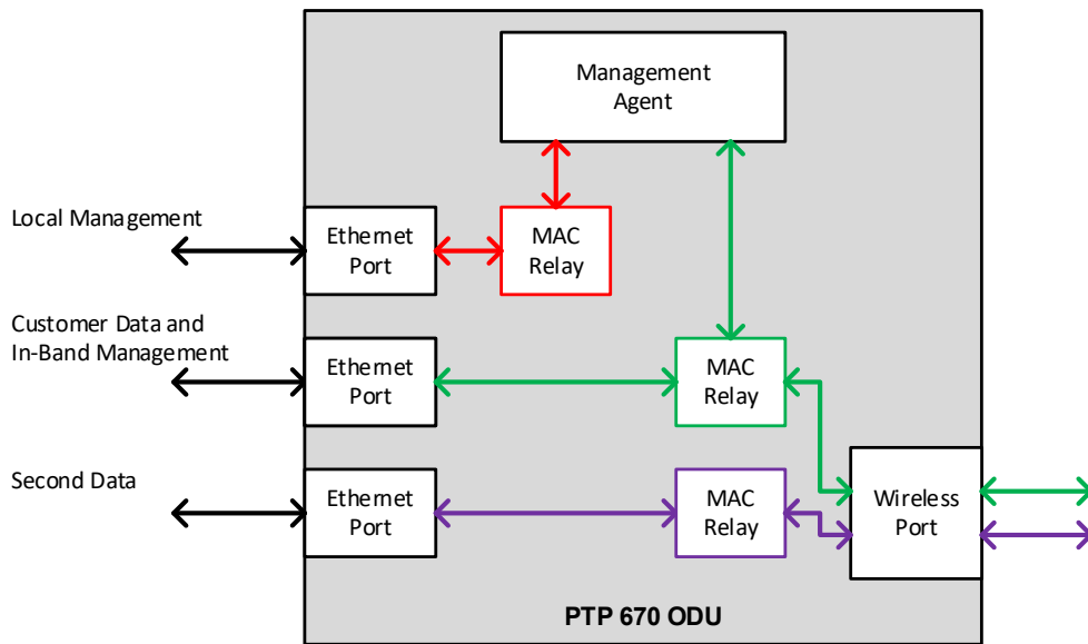
Figure 52 Ports and Services: Data + Second Data + In-Band Management (with Data) + Local Management
