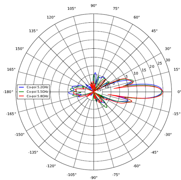
H-POL AZIMUTH GAIN (dBi) FOR ZERO ELEVATION
