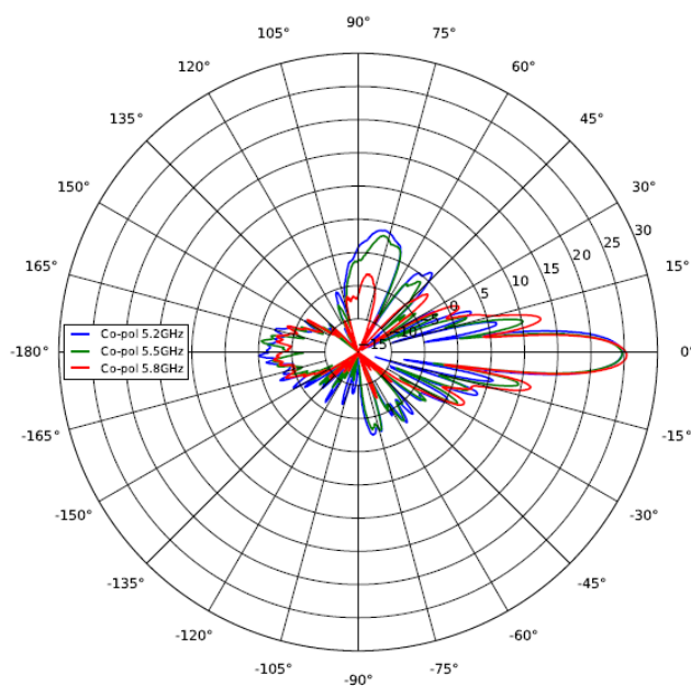
H-POL ELEVATION GAIN (dBi) FOR ZERO AZIMUTH
