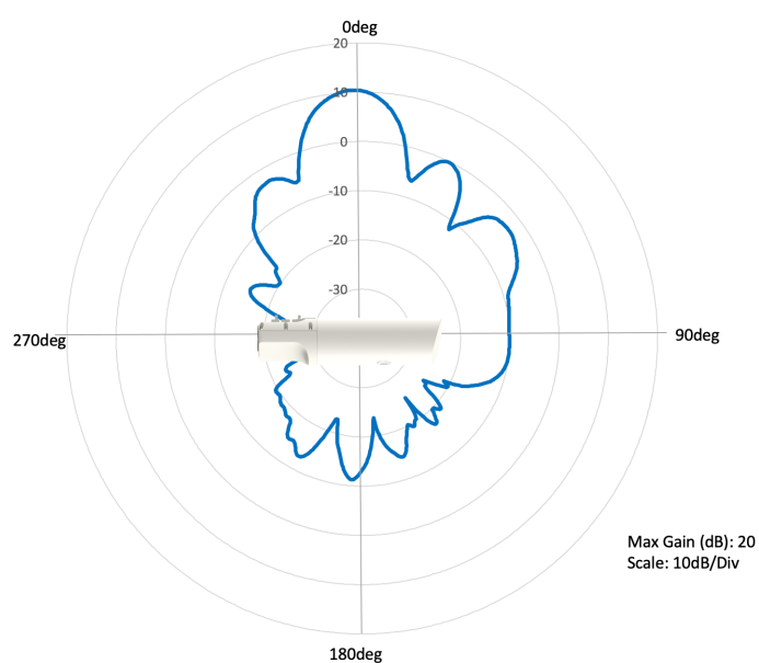
2.4 GHz Elevation
