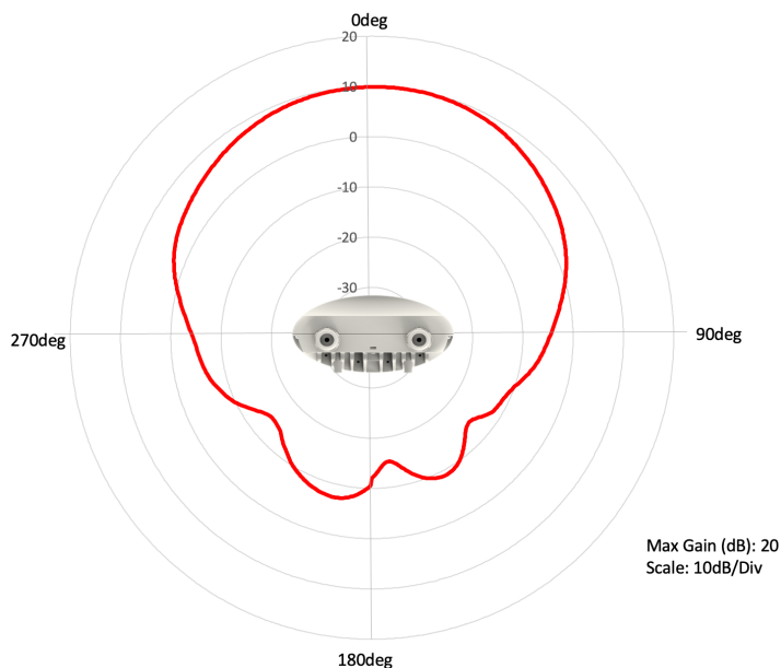
2.4 GHz Azimuth
