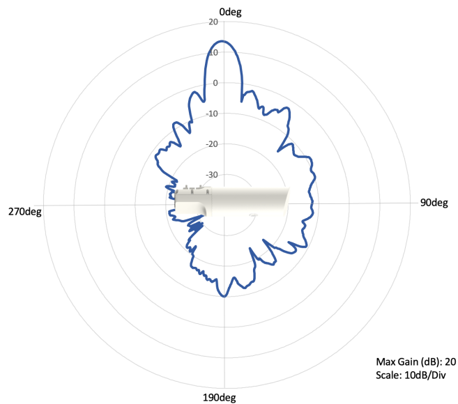
5 GHz Elevation
