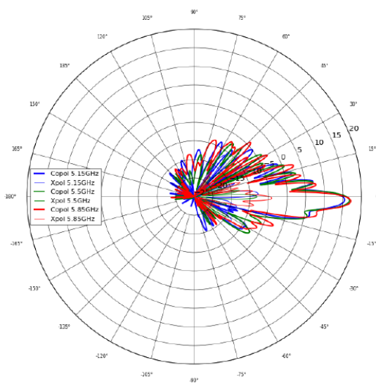
CH 0 Vertical Polarization, Elevation
