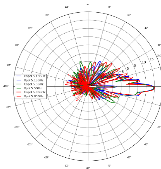
CH 6 Vertical Polarization, Elevation
