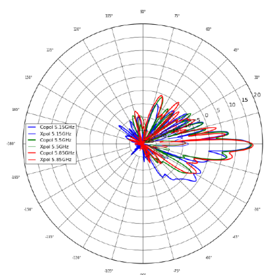
CH 5 Vertical Polarization, Elevation
