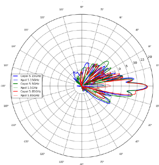
CH 4 Vertical Polarization, Elevation
