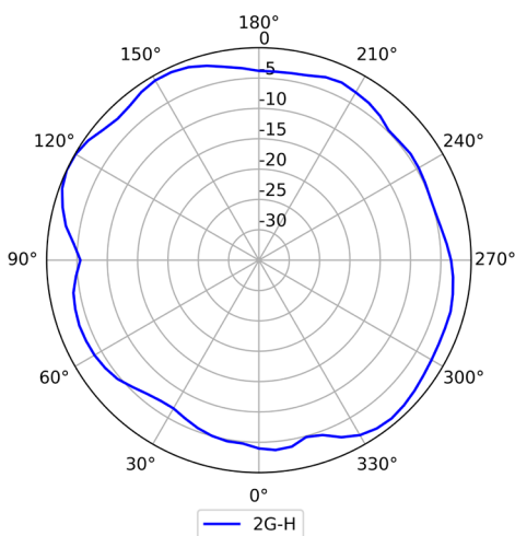
2.4G (Horizontal)
