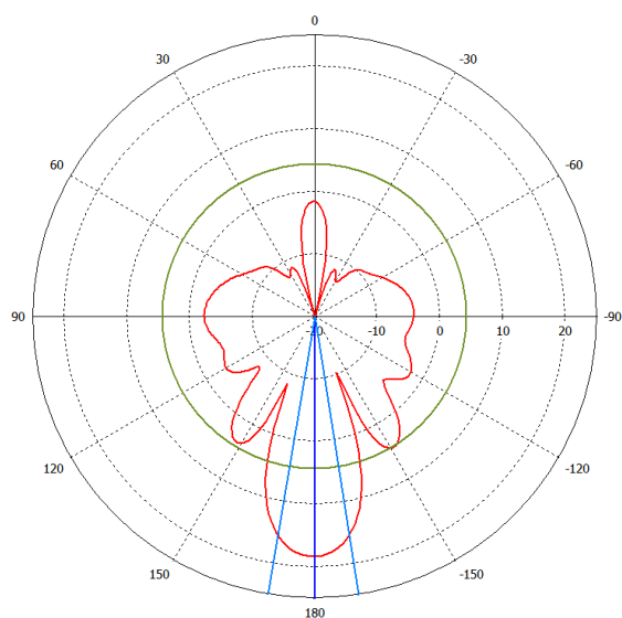
Horizontal 0 deg
