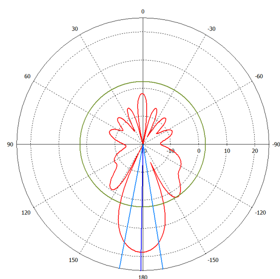
Vertical 0 deg
