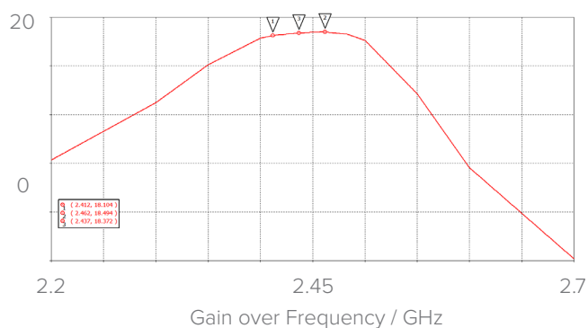
Vertical polarization
