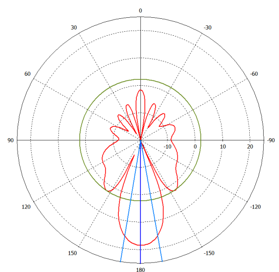
Horizontal 90 deg
