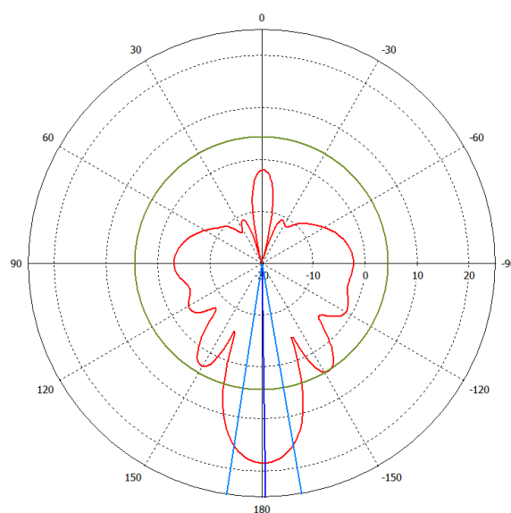
Vertical 90 deg
