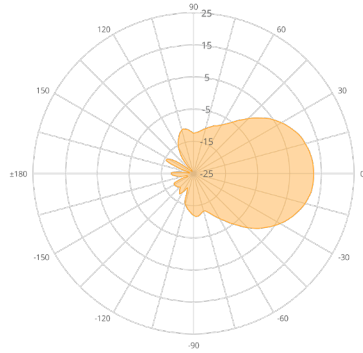
N5-X12 (12 dBi)
