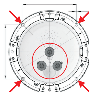
Drill the holes
