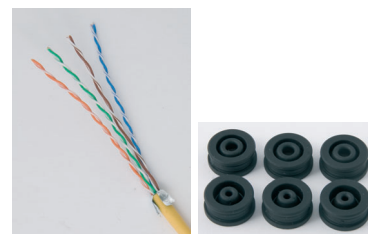
Prepare the Ethernet cable: remove insulation, shorten sheath and fold back over insulation, push rubber seal over cable
