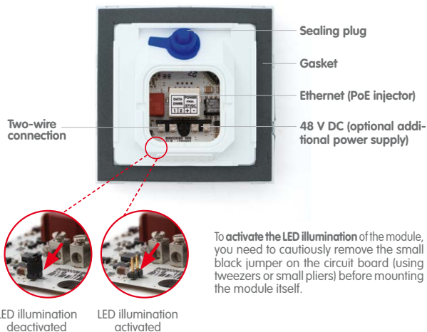
View with housing cover removed
