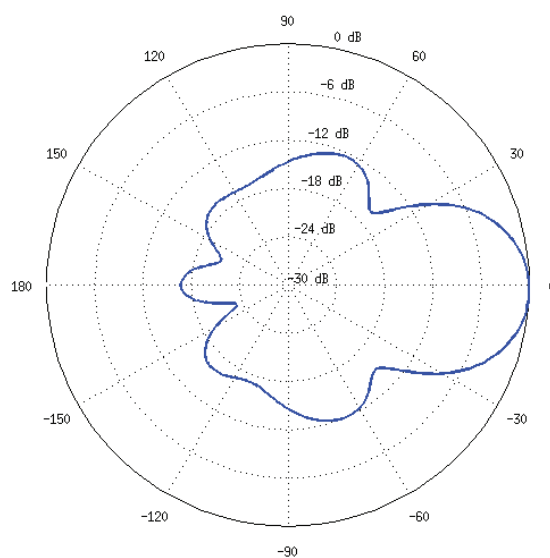
Horizontal Elevation
