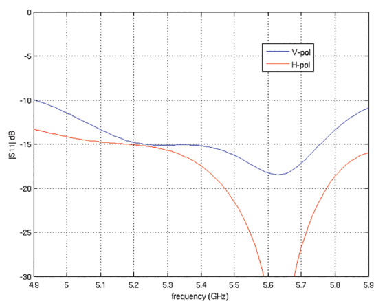
Return Loss
