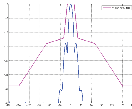
Elevation Specs
