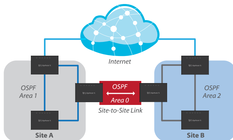
Example of a Service Provider Deployment for the ER-X
