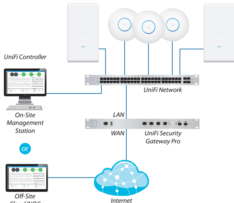
Example of a UniFi Enterprise System
