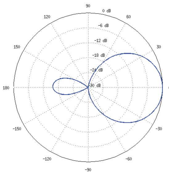
Horizontal Elevation
