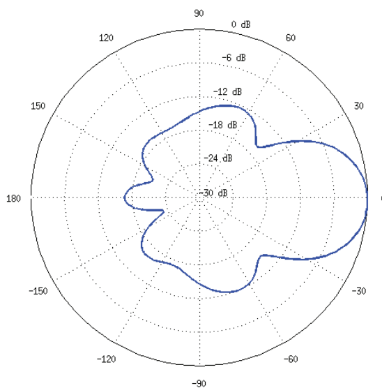
Vertical Elevation
